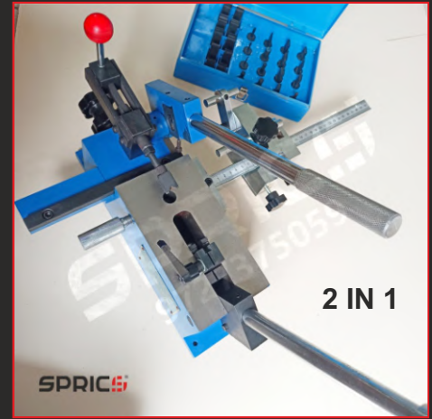
LABEL RULE (2 in 1) BENDING MACHINE 8MM - 12MM
