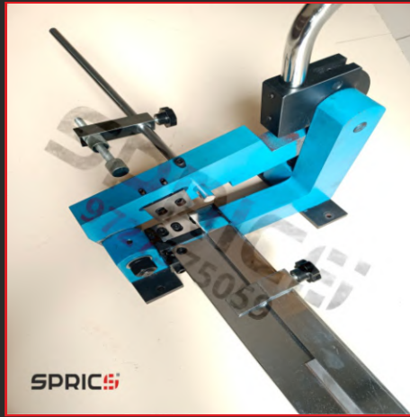
CUTTING & LIPPING MACHINE Max. Thickness: 2 MM Max. Width: 40 MM
